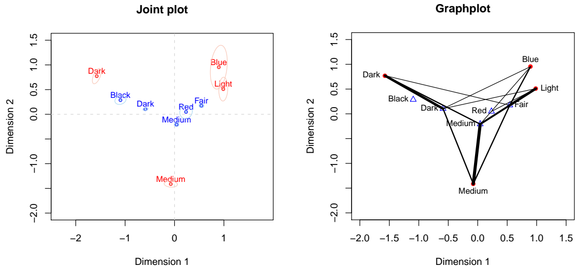
Figure 1: Joint plot and graph plot for Tocher data.
