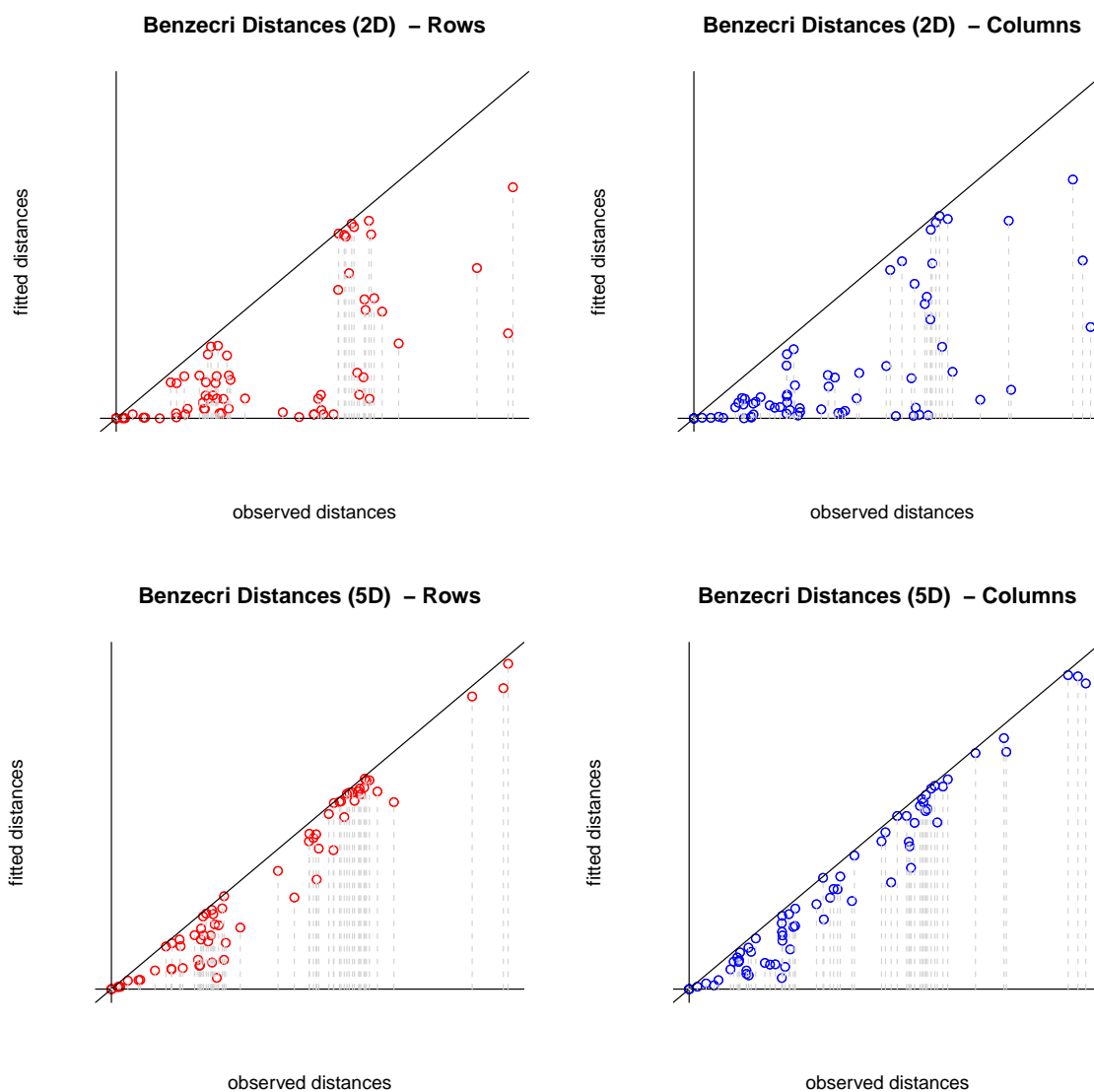
Figure 2: Benzécri plots for Bitterling data.
