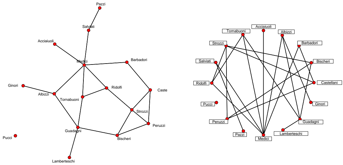
Figure 1: Sample displays of the Florentine marriage data; the left panel depicts the default Fruchterman-Reingold layout, while the right panel depicts a circular layout.
