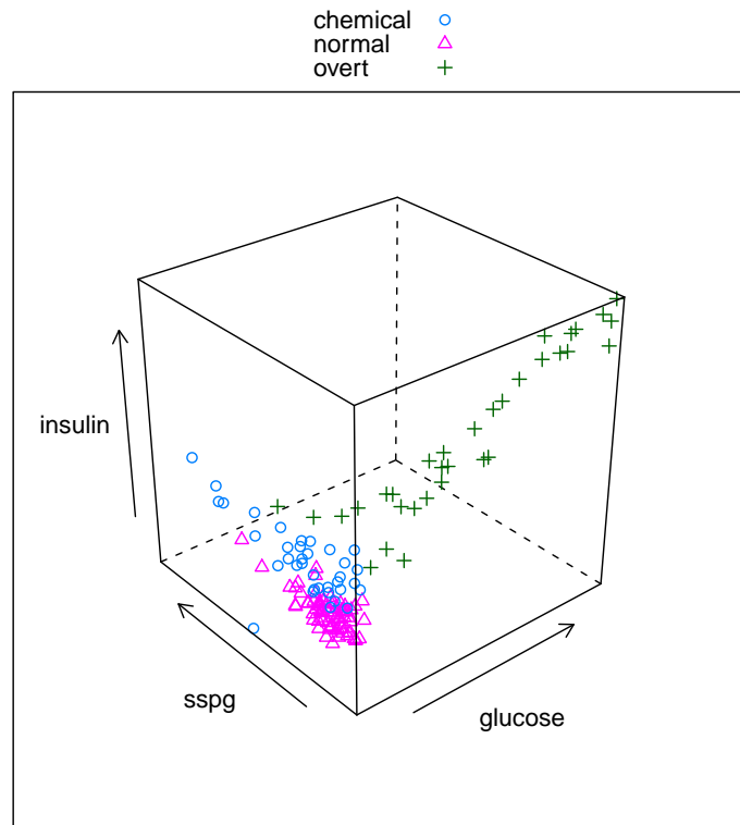
Figure 15: 3-dimensional scatter plot of the diabetes data.
