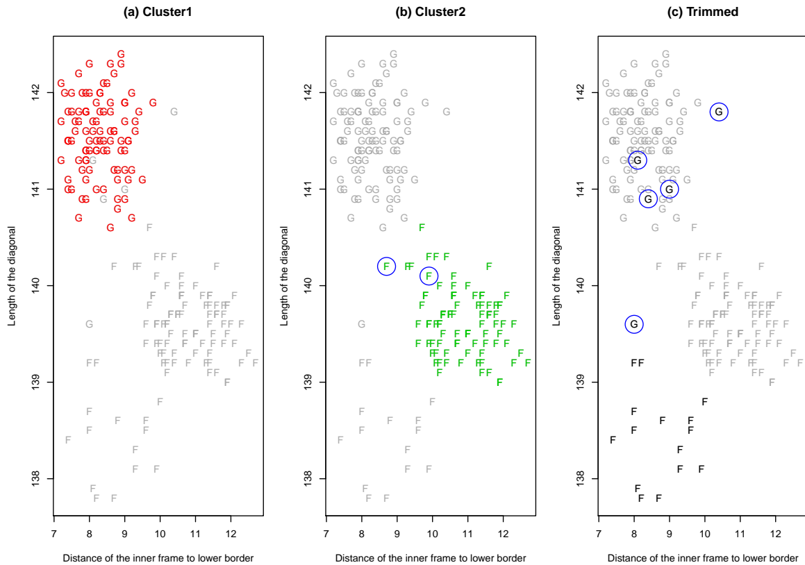
Figure 14: Clustering results with k = 2 , \alpha = 0.1 and restr.fact = 50 for the “Swiss Bank notes” data set. Only the fourth and sixth variables are plotted. The 7 most doubtful decisions are rounded by a circle symbol.
