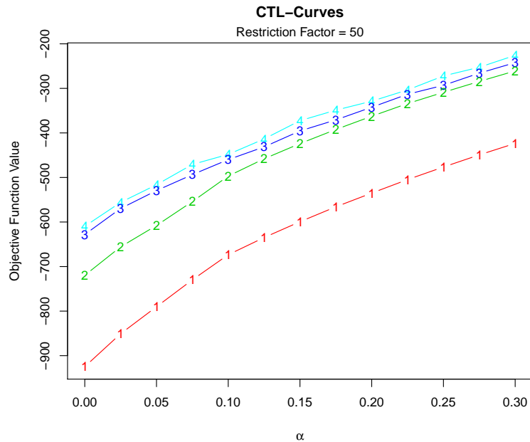
Figure 12: Classification trimmed likelihoods for k = 1, \dots, 4 and \alpha = 0, 0.025, \dots, 0.3 when restr.fact = 50 for the “Swiss Bank notes” data set.
