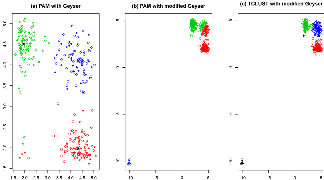
Figure 5: PAM’s clustering results for the geyser2 data with 3-medoids denoted by the symbol “ x ” in (a). PAM’s clustering results for a modified geyser2 data set in (b) and when applying tkmeans with k = 3 and \alpha = 0.03 in (c).
