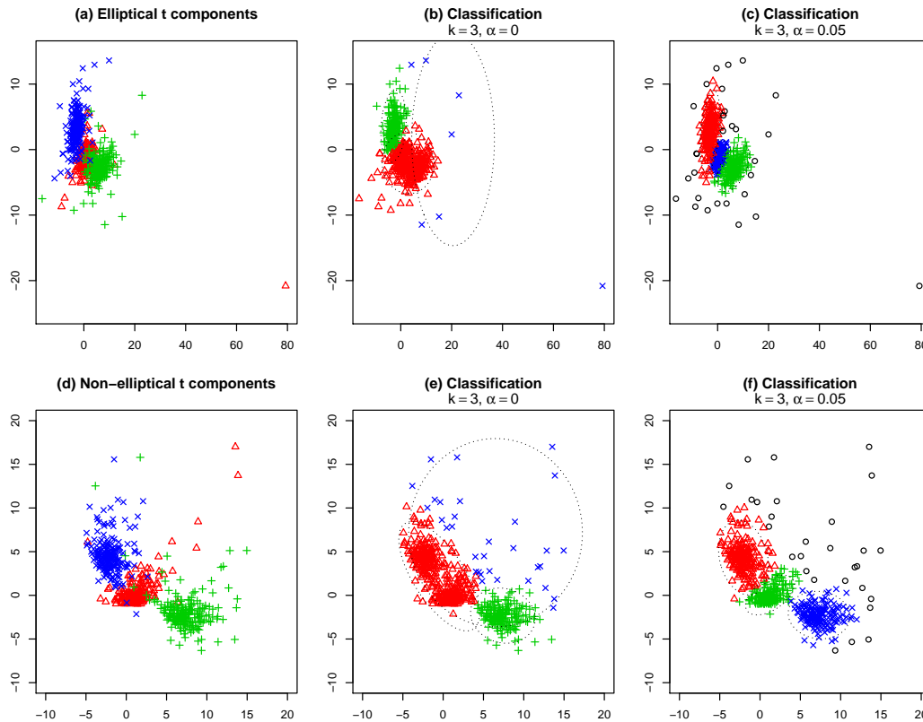
Figure 6: A data set made up of three elliptical t components is shown in (a) and three asymmetrical t components in (d). The associated clustering results when applying the tclust function with k = 3 and \alpha = 0 are shown in (b) and (e) and with k = 3 and \alpha = 0.05 in (c) and (f).
