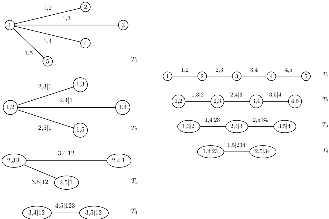
Figure 1: Examples of five-dimensional C- (left panel) and D-vine trees (right panel) with edge indices.
