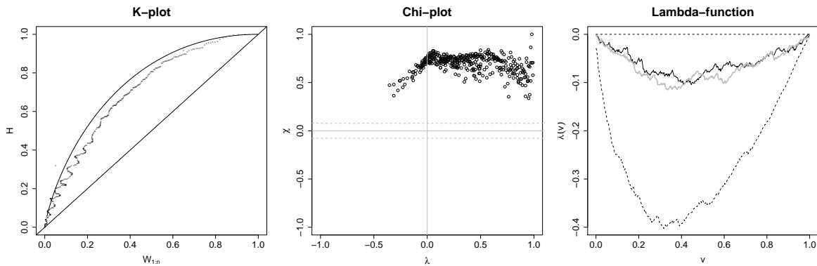
Figure 8: Left panel: K-plot. Middle panel: chi-plot. Right panel: empirical \lambda -function (black line), theoretical \lambda -function of a Student- t copula with parameters estimated using BiCopEst (grey line) as well as independence and comonotonicity limits (dashed lines). Code for this plot is given in the replication file.
