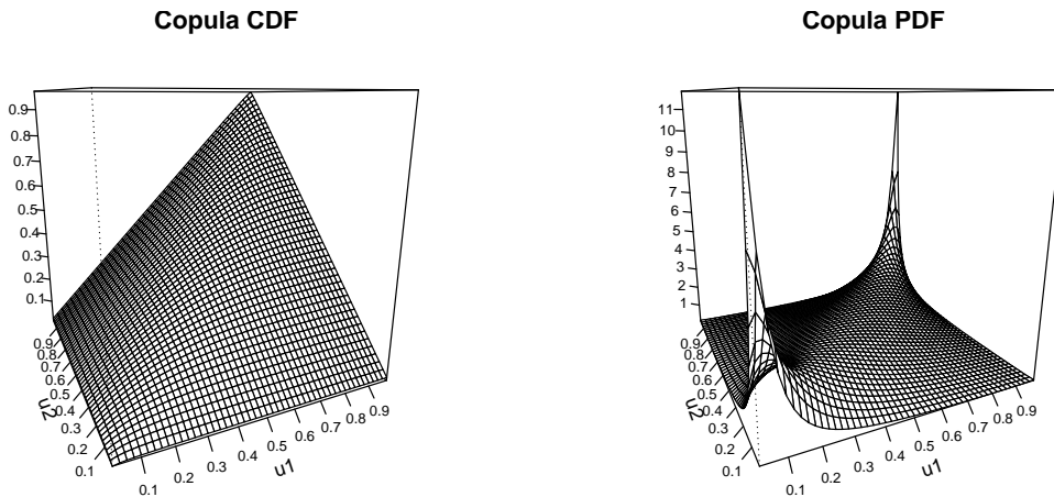
Figure 3: CDF and PDF of a bivariate Student- t copula with dependence parameter \rho = 0.7 and 4 degrees of freedom.
