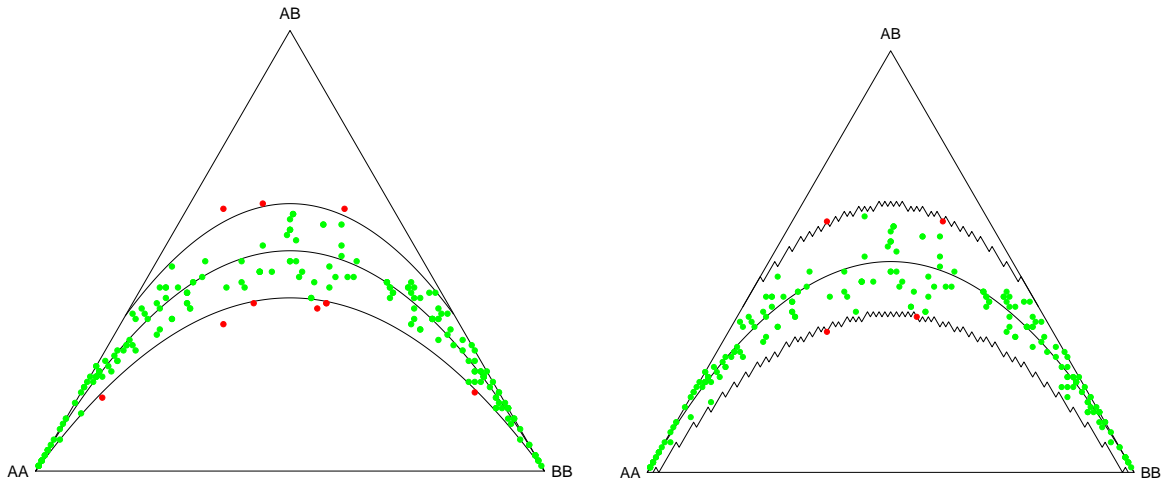
Figure 7: Ternary plots of 225 SNPs on chromosome 1 of a sample of 84 individuals from a Han Chinese population. Left: Ternary plot with the acceptance region of a chi-square test. Right: Ternary plot with the acceptance region of an exact test.
