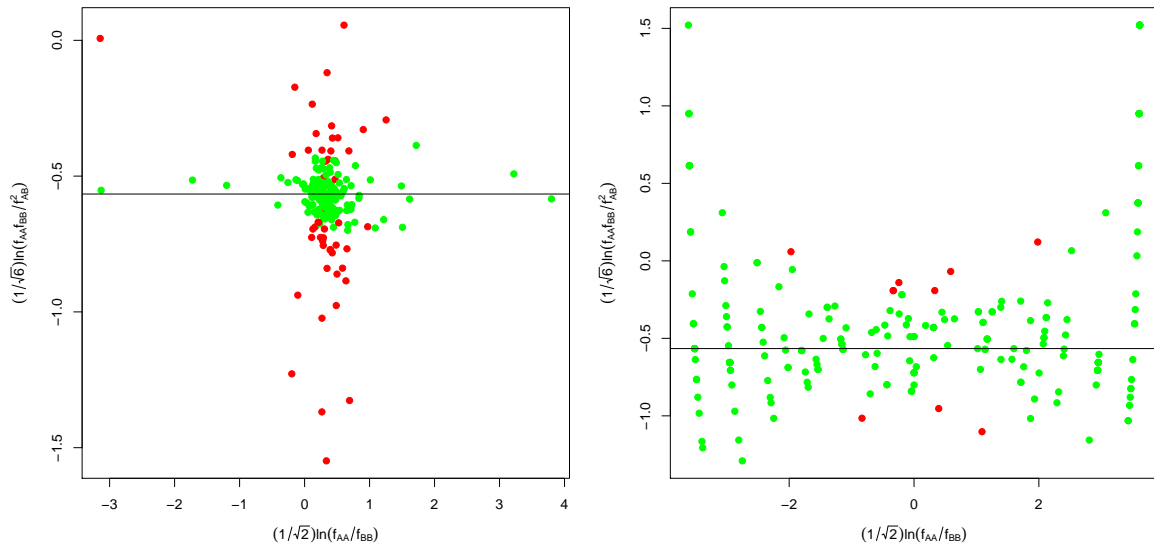
Figure 4: Left: ilr plot of MN blood group genotype frequencies for 216 samples from different human populations. Right: ilr plot for 225 SNPs on chromosome 1 of a sample of 84 individuals from a Han Chinese population. HWE is represented by the horizontal line with ordinate -\sqrt{2/3}\ln(2) = -0.57 . Markers are colored according to a chi-square test for HWE (red points significant, green points not significant).
