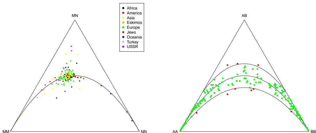
Figure 3: Left: Ternary plot for one marker: MN blood group genotype frequencies for 216 samples from different human populations. Right: Ternary plot for multiple markers: 225 SNPs on chromosome 1 of a sample of 84 individuals from the Han Chinese population. HWE parabola and acceptance region for a chi-square test are shown in the latter plot.
