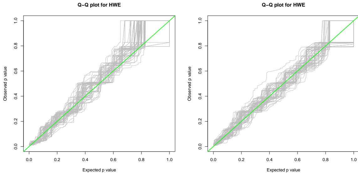
Figure 8: Left: Q-Q plot for 225 SNPs on chromosome 1 of a sample of 84 individuals from the Han Chinese population. Right: Q-Q plot for simulated data (225 SNPs, 84 individuals, matched in allele frequency).
