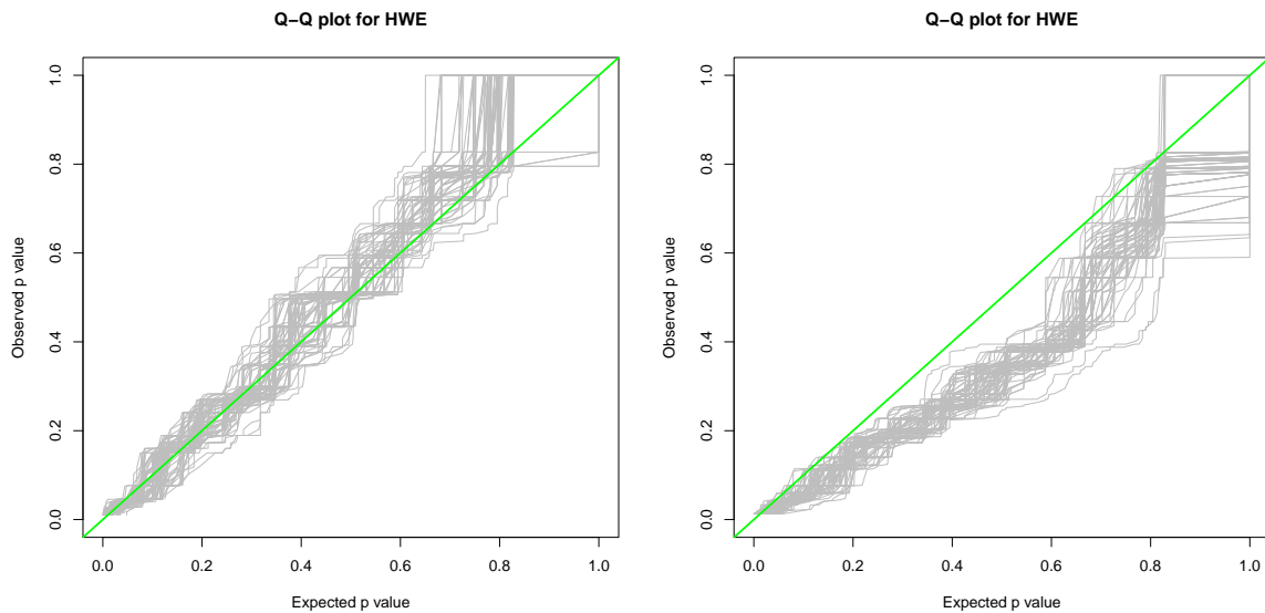
Figure 5: Left: Q-Q plot for 225 SNPs on chromosome 1 of a sample of 84 individuals from the Han Chinese population. Right: Q-Q plot for simulated data (225 SNPs, 84 individuals) with inbreeding ( f = 0.05 ).
