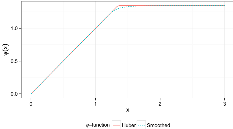
Figure 3: Comparison of the Huber and the smoothed Huber \psi -function for k = 1.345 and s = 10 .
