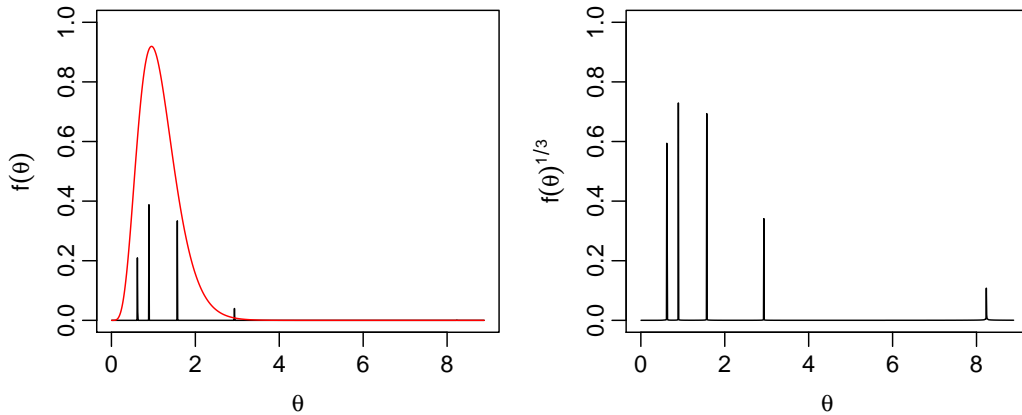
Figure 4: Estimated mixing distribution G for \theta for the group insurance data. The left panel depicts to the Kiefer-Wolfowitz NPMLE estimator for G with 1000 grid points. The right panel depicts the cube root of the mass associated with support points around 8. The smooth curve superimposed in the left panel corresponds to the parametric maximum likelihood estimate of the mixing density assuming G follows a Gamma distribution.
