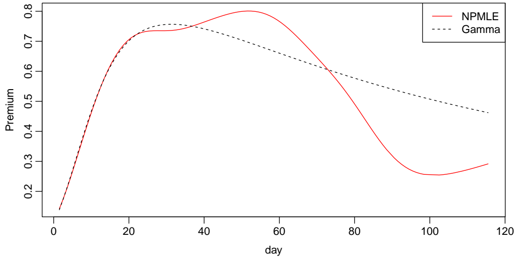
Figure 10: Ten-day term life insurance premia for medflies of various ages.
