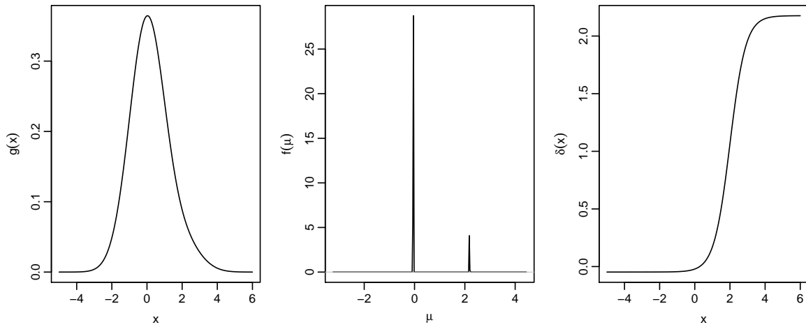
Figure 1: Kiefer-Wolfowitz estimation of a Gaussian location mixture: The left panel is the (unknown) two component mixture density, the middle panel is the estimated NPMLE mixing density and the right panel is the estimated Bayes rule for predicting \hat{\mu} = \delta(x) based on seeing an observation x .
