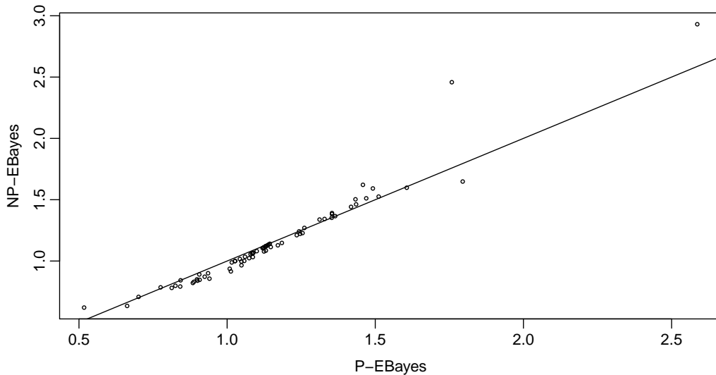
Figure 5: Comparison of the Parametric and the Nonparametric Empirical Bayes estimator of \theta_i for 72 occupation groups. As indicated by the 45 degree line there is good agreement between the parametric and nonparametric Bayes rules except for the two groups appearing in the upper right corner of the plot.
