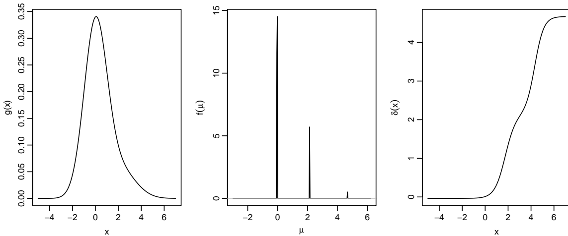
Figure 2: Kiefer-Wolfowitz estimation of a Gaussian location mixture: The left panel is the (unknown) mixture density, the middle panel is the estimated NPMLE mixing density and the right panel is the estimated Bayes rule for predicting \hat{\mu} = \delta(x) based on seeing an observation x .
