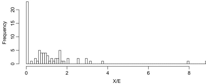
Figure 3: Histogram of claims per exposure for 72 occupation groups.
