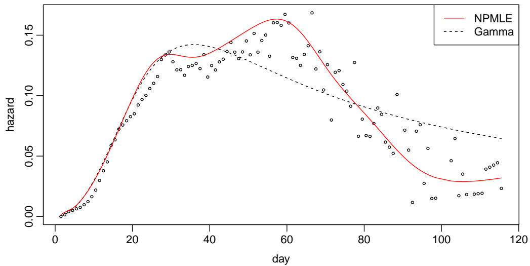
Figure 8: Parametric versus nonparametric estimates of medfly mortality rates.
