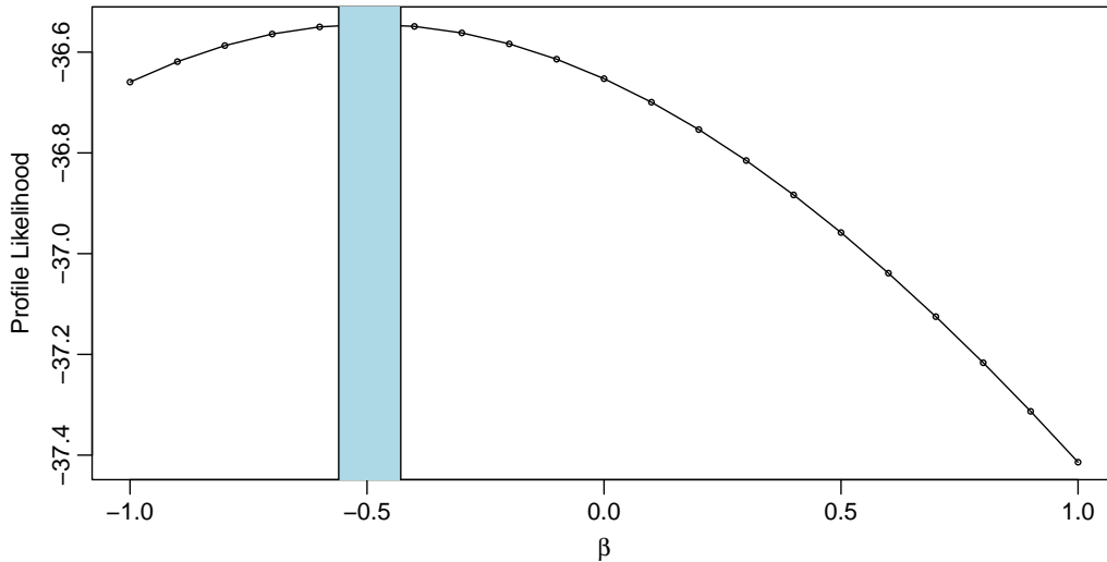
Figure 7: Initial cage density effect in the Weibull mixture model: Profile log likelihood (in 1000s) for the cage density effect with 0.95 (Wilks) confidence interval in blue.
