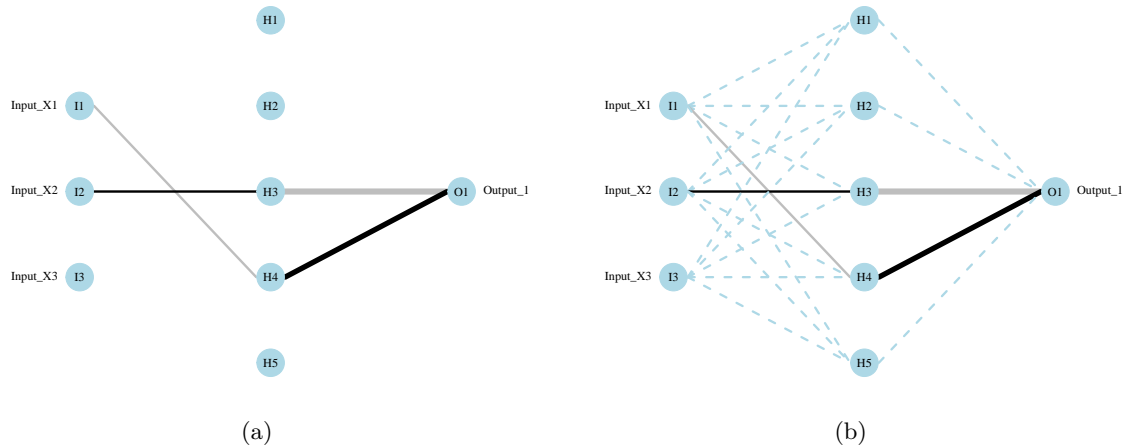
Figure 3: A pruned neural network from RSNNS (Bergmeir and Benítez 2012) using the “optimal brain surgeon” algorithm described in Zell et al. (1998). The default plotting behavior of plotnet is to omit pruned connections (3a), whereas they can be viewed as dashed lines by including the prune_col argument (3b).
