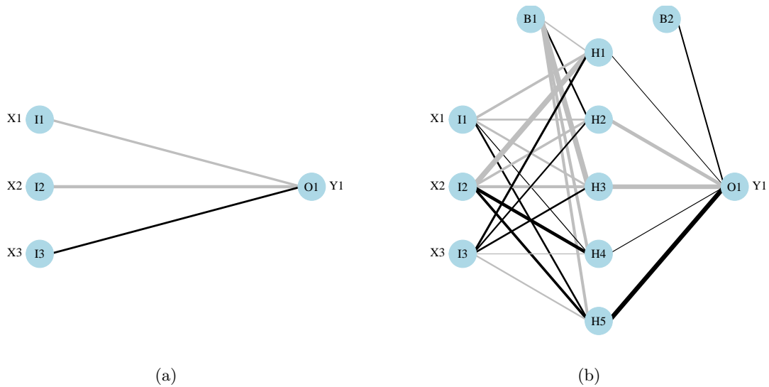
Figure 2: Examples from the plotnet function showing a neural network with a separate skip layer between the input and output layers. The skip layer (2a) and primary neural network (2b) can be viewed separately with plotnet by using skip = TRUE or skip = FALSE .
