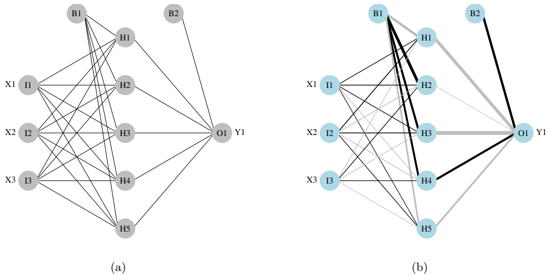
Figure 1: Examples from the plotnet function showing neural networks as a standard graphic (1a) and using the neural interpretation diagram (1b). Labels outside of the nodes represent variable names and labels within the nodes indicate the layer and node (I: input, H: hidden, O: output, B: bias).
