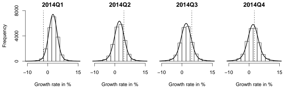
Figure 4: Forecast distributions for the growth rate of US GDP. The forecasts stem from a Bayesian time series model, as detailed in Krüger et al. (2016, Section 5). Histograms summarize simulated forecast draws at each date. Mixture-of-normals approximation to distribution shown in black; realizing observations shown by dashed line.
