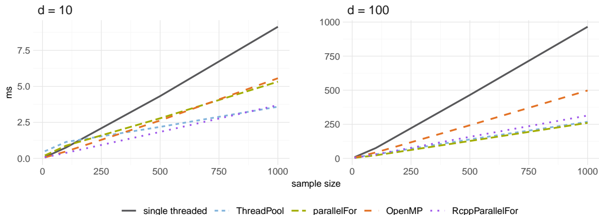
Figure 5: Time required for computing Kendall's correlation matrix in parallel for d variables.
