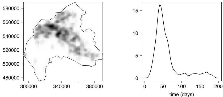
Figure 5: Spatial (left) and temporal (right) intensity functions estimated from the fmd dataset.
