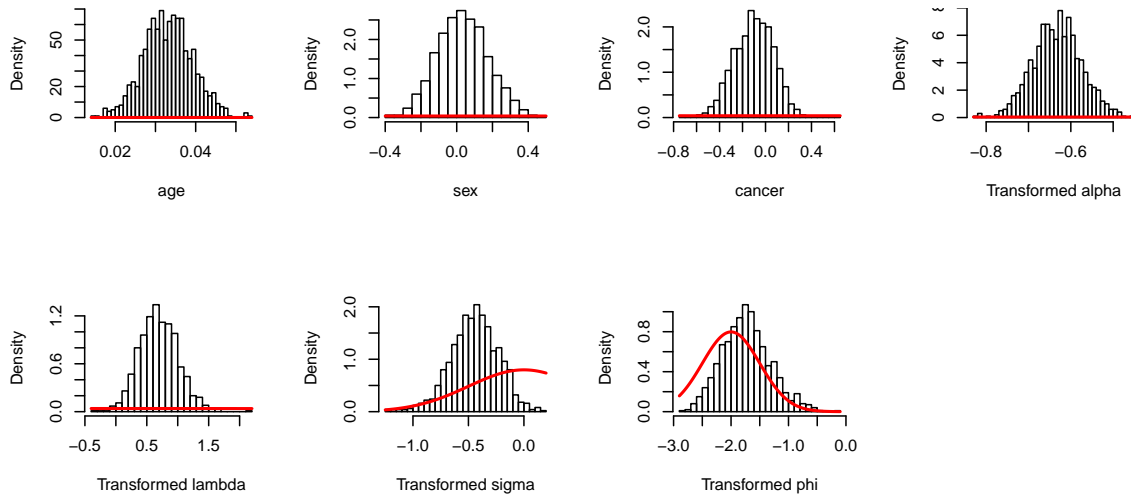
Figure 5: Plot showing the prior (red line) and posterior (histogram) for each parameter. At this scale, the priors for \beta and \omega appear as flat lines, this is because they are uninformative.
