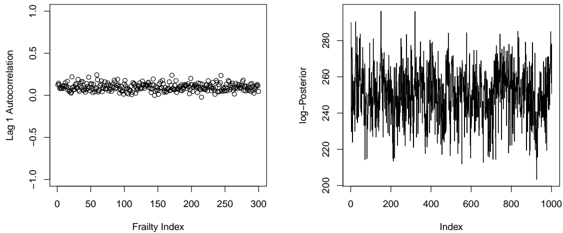
Figure 4: Left: Lag-1 autocorrelations in the Y chains. Right: Plot of the log-posterior.
