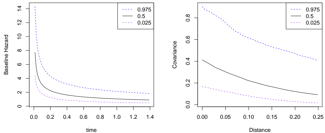
Figure 6: Left: Plot showing the posterior median baseline hazard and 95% credible interval. Right: Plot showing the posterior median of the spatial covariance function and 95% credible interval.
