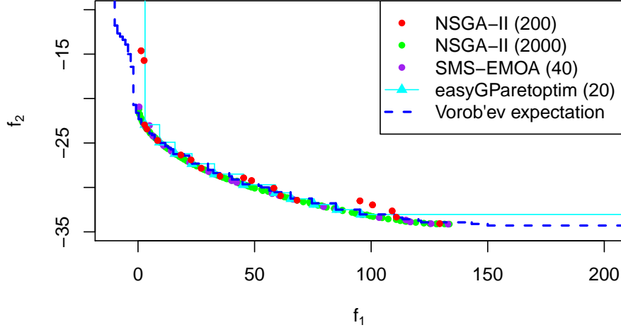
Figure 8: Comparison of four algorithms to find the Pareto front of Example 2.
