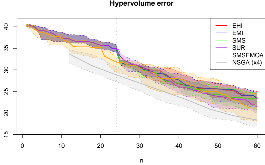
Figure 10: Evolution of hypervolume error with respect to a reference Pareto front for the problem ( P2 ). Representation is similar to Figure 9 except that for NSGA-II, where the number of observations is to be multiplied by 4.
