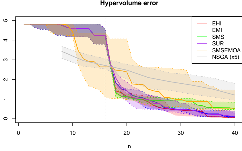
Figure 9: Evolution of hypervolume error with respect to a reference Pareto front for problem ZDT3 for various infill criteria over 25 repetitions. Curves are for the median performance and dotted lines denote the first and third quartiles. For NSGA-II, the number of observations is to be multiplied by five.
